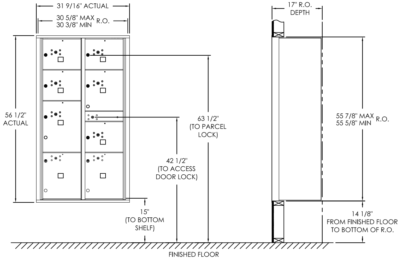
COMPARTMENT CHART
